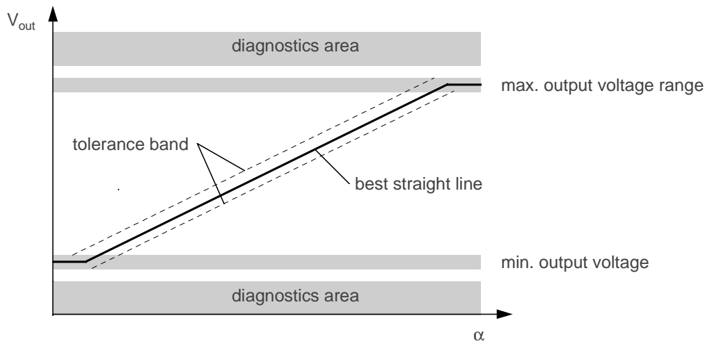
Figure 6: UZZ9000 output characteristic
