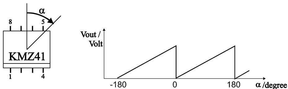
Figure 17: Definition of mechanical angle and the resulting output curve characteristic when using the standard connection between KMZ41 and UZZ9000
